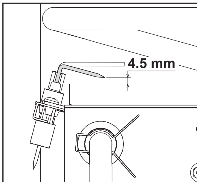
fig. 16 - Electrode position
