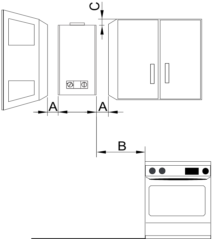
fig. 5 - Minimum distances
